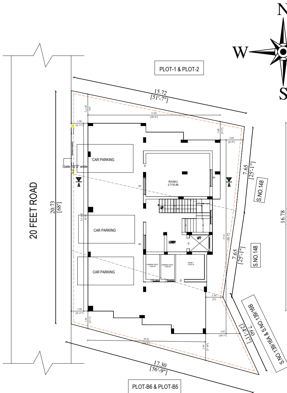
PRO SITE CUM STILT FLOOR PLAN
