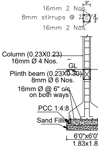
FOUNDATION DETAIL
