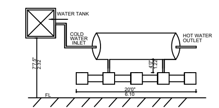
SOLOR HOT WATER SYSTEM DETAILS
