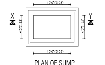
PLAN OF SUMP
