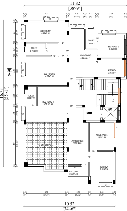
PRO.THIRD FLOOR PLAN
