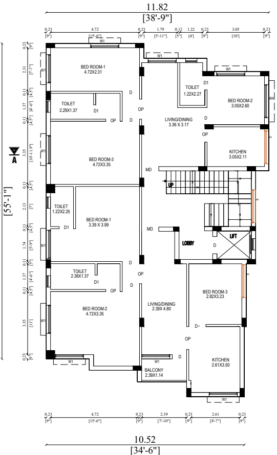
PRO.SECOND FLOOR PLAN
