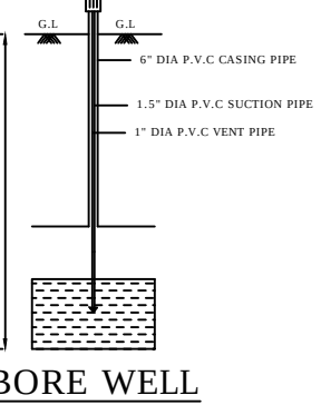
BORE WELL
