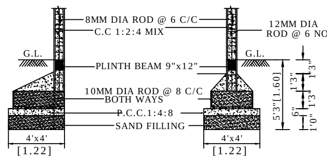
RUN THROUGH COLUMN FOUNDATION SCALE 1" = 4'0" (1:50)
