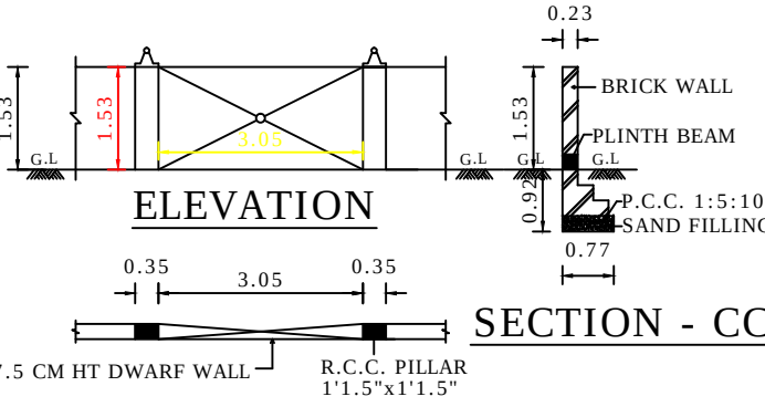
COMPOUND WALL PLAN
