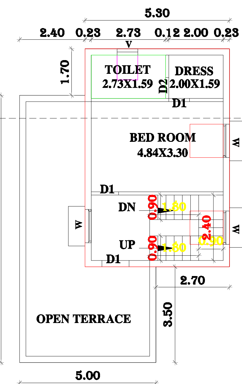
FIRST FLOOR PLAN PROPOSED
