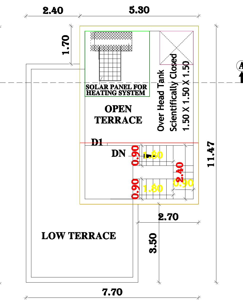
TERRACE FLOOR PLAN PROPOSED
