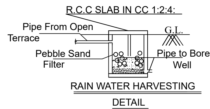
RAIN WATER HARVESTING DETAIL
