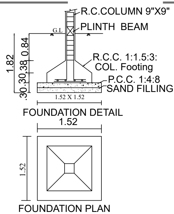
FOUNDATION PLAN
