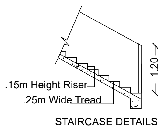
STAIRCASE DETAILS
