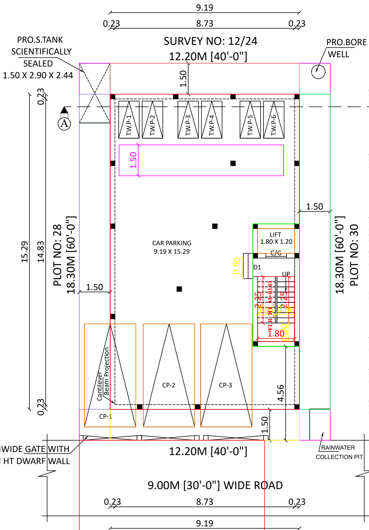
SITE CUM PRO.STILT FLOOR PLAN
