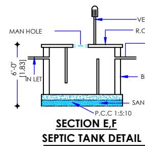
SECTION E.F. SEPTIC TANK DETAIL
