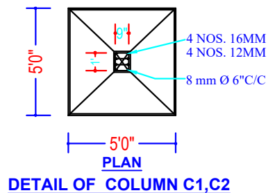
DETAIL OF COLUMN C1,C2
