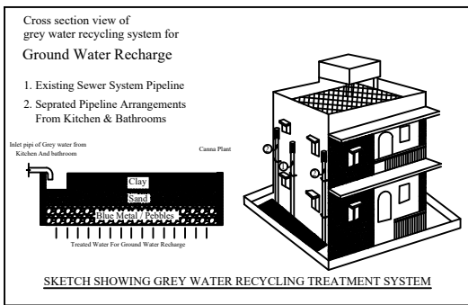
SKETCH SHOWING GREY WATER RECYCLING TREATMENT SYSTEM
