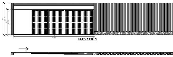
PLAN COMPOUND WALL DETAIL
