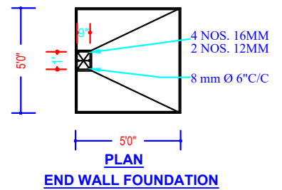
END WALL FOUNDATION
