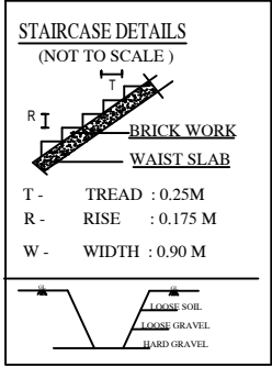
STAIRCASE DETAILS
