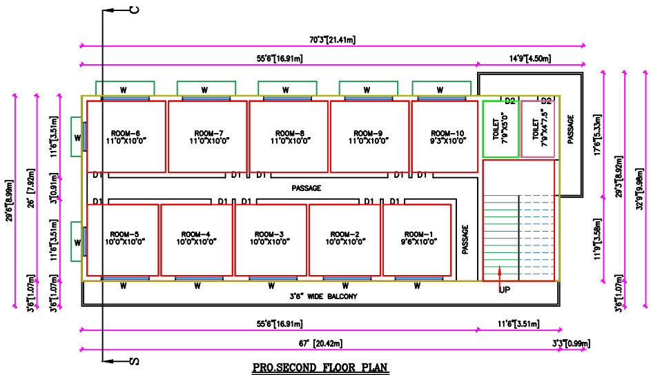
PRO. SECOND FLOOR PLAN
