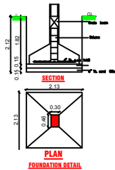
FOUNDATION DETAIL
