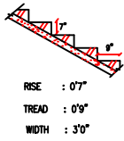
STAIRS DETAILS
