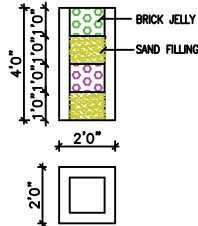
PERCOLATION PIT
