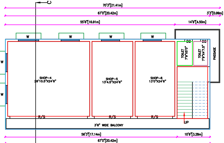
EXTG. FIRST FLOOR PLAN
