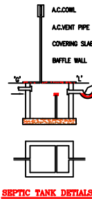
SEPTIC TANK DETAILS
