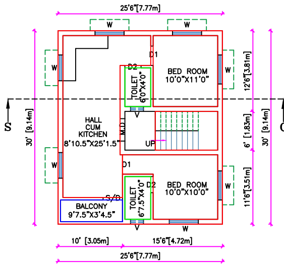
PRO. SECOND FLOOR PLAN
