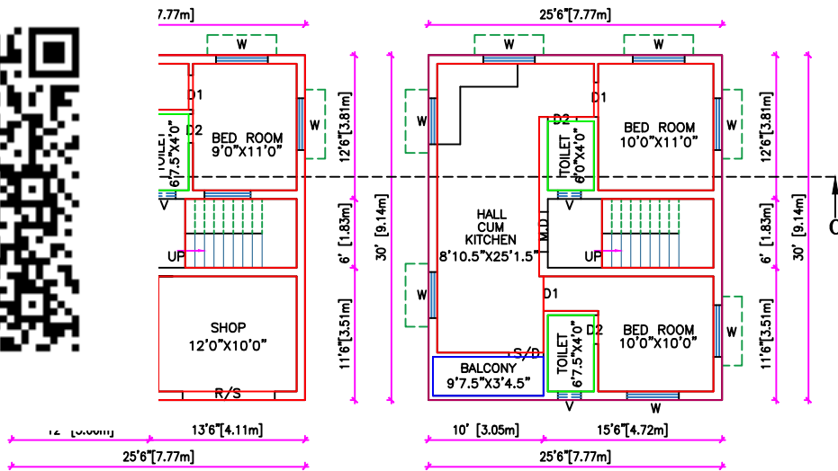
EXT. GROUND FLOOR PLAN
