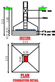
PLAN FOUNDATION DETAIL
