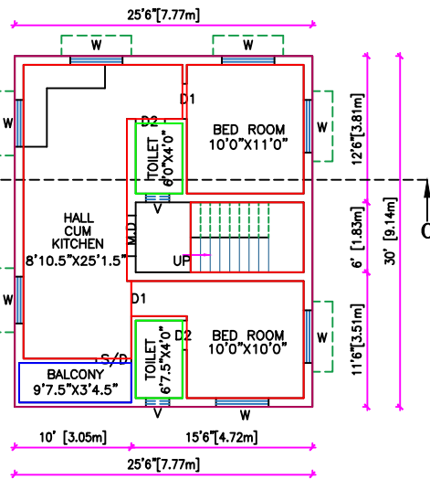
EXT. FIRST FLOOR PLAN
