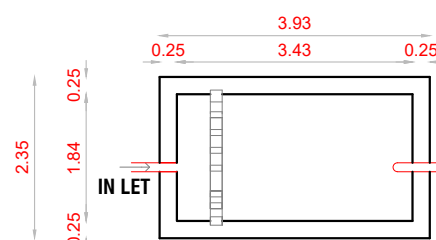
PLAN OF SEPTIC TANK CAPACITY - 8000 LITRES
