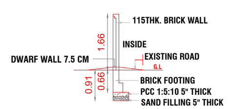
SECTION OF COMPOUND WALL
