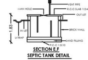
SECTION E-F SEPTIC TANK DETAIL
