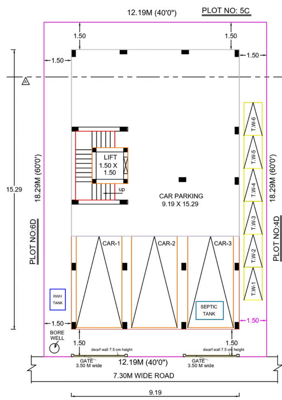
SITE CUM STILT FLOOR PLAN
