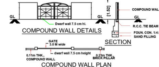
COMPOUND WALL PLAN
