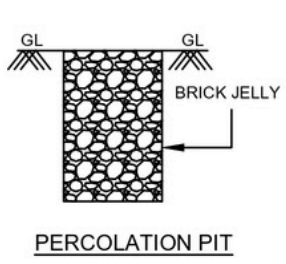
PERCOLATION PIT
