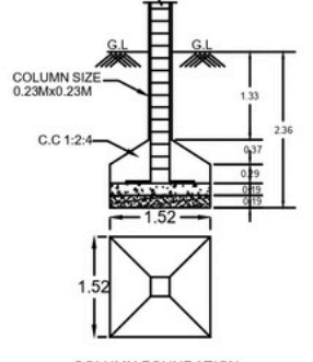
COLUMN FOUNDATION
