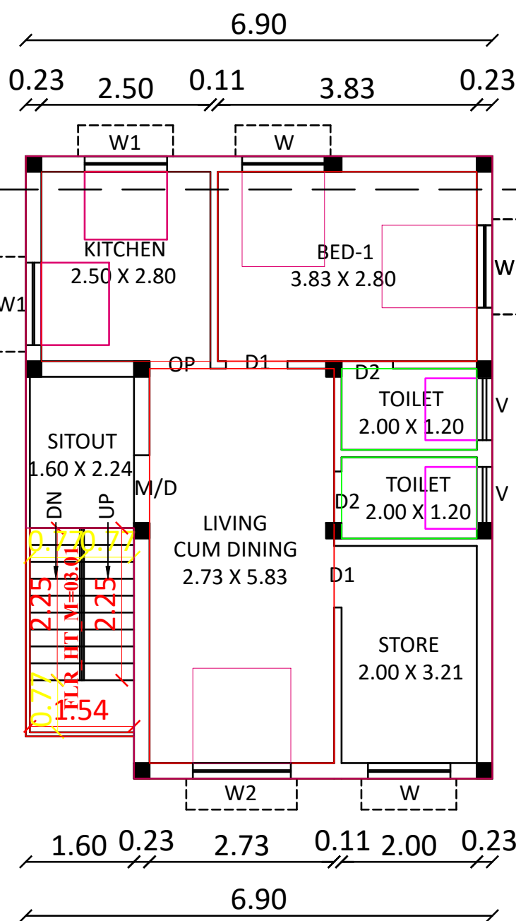
PRO.SECOND FLOOR PLAN
