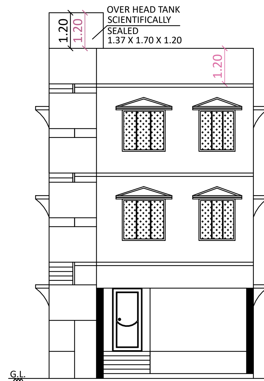
FRONT ELEVATION
