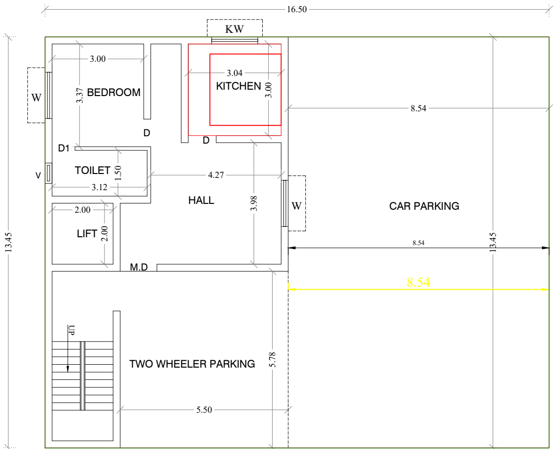
PRO. GROUND FLOOR PLAN
