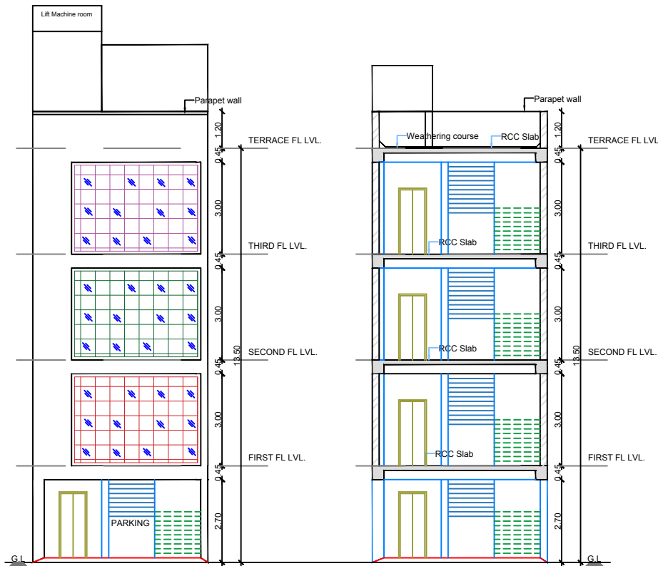
FRONT ELEVATION
