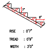
STAIRS DETAILS
