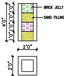
PERCOLATION PIT
