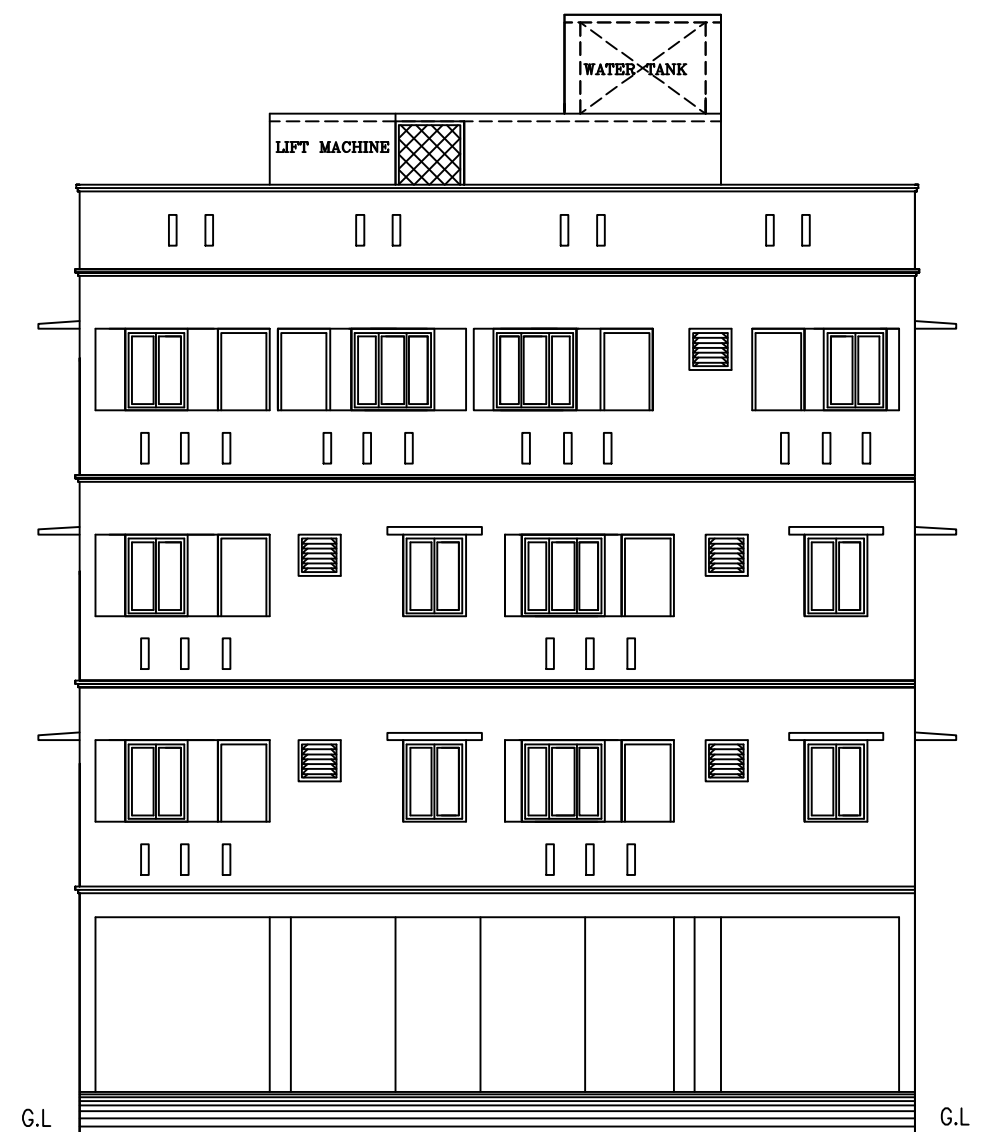
FRONT ELEVATION
