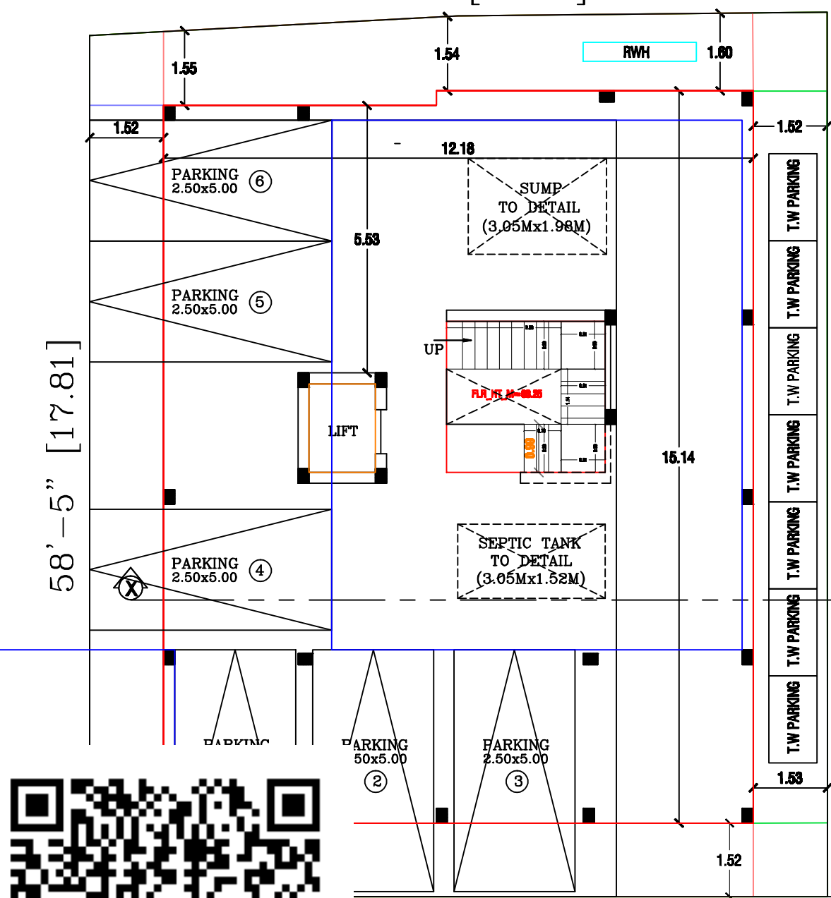
STILT FLOOR PLAN (PROPOSED)
