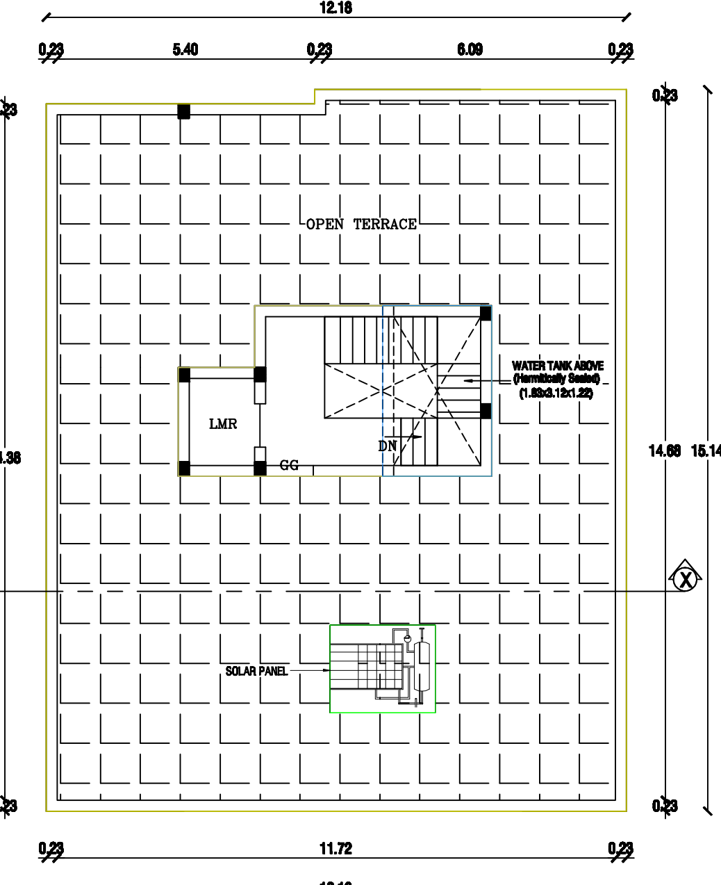
TERRACE FLOOR PLAN (PROPOSED)
