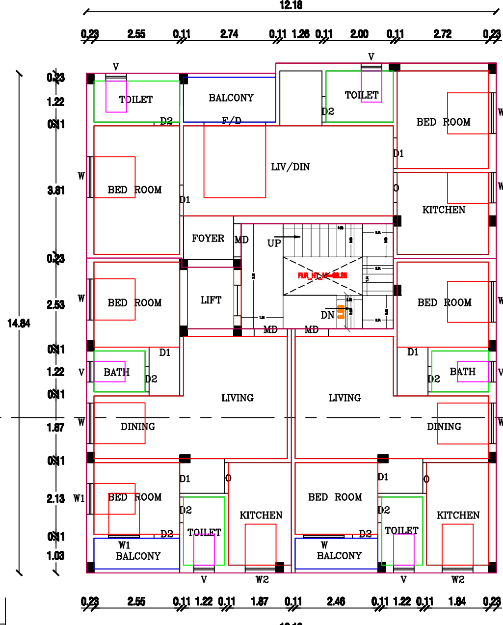
FIRST AND SCND FLOOR PLAN (PROPOSED)
