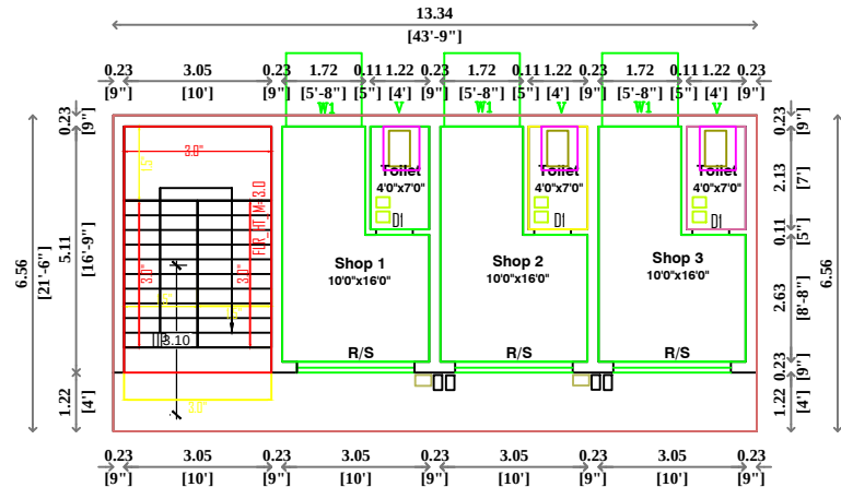
PROPOSED FIRST FLOOR PLAN (COMMERCIAL)
