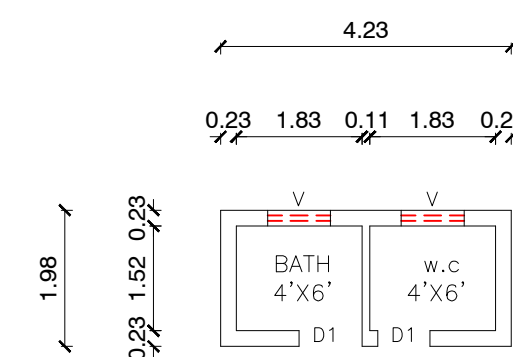
PROPOSED TOILET PLAN
