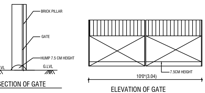
ELEVATION OF GATE
