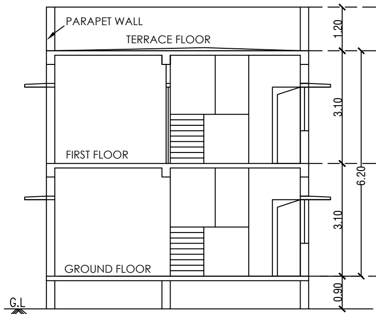
SECTION 'X-X'
