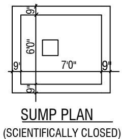
SUMP PLAN (SCIENTIFICALLY CLOSED)
