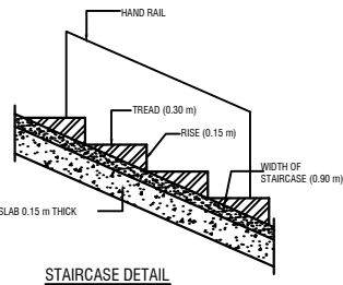
STAIRCASE DETAIL
