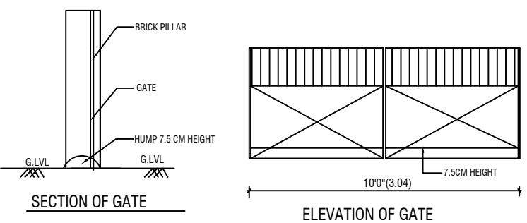
ELEVATION OF GATE
