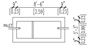
DETAILS OF SEPTIC TANK
