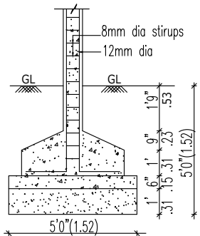
COLUMN FOUNDATION DETAIL
