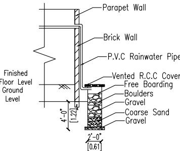
SECTION OF RAINWATER HARVESTING SYSTEM PERCOLATION TRENCH METHOD
