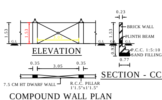
COMPOUND WALL PLAN
