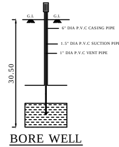
BORE WELL
