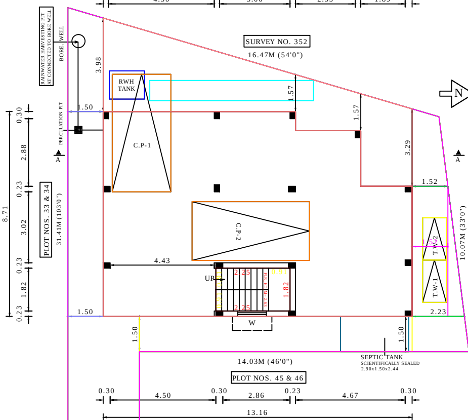
SITE CUM STILT FLOOR PLAN
