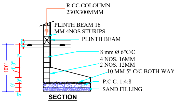
SECTION
