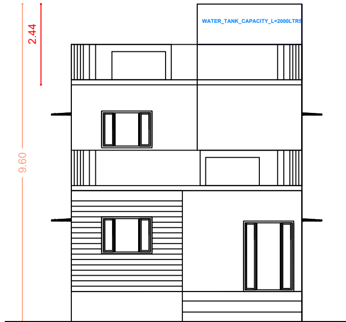
FRONT ELEVATION
