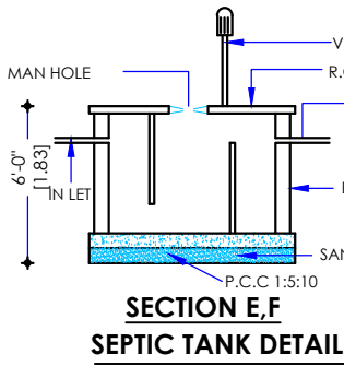
SECTION E,F SEPTIC TANK DETAIL
