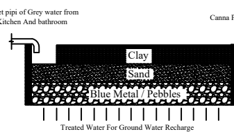
SKETCH SHOWING GREY WATER RECYCLING TREATMENT SYSTEM
