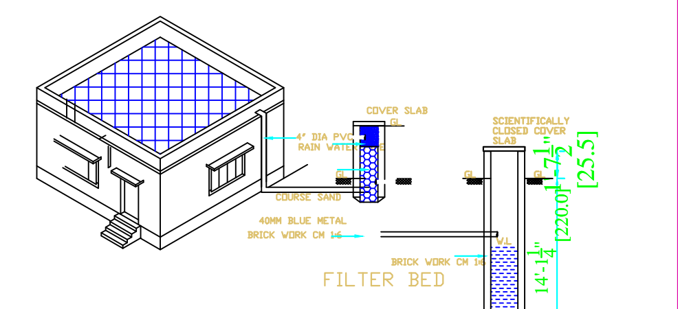
PROPOSED RAIN WATER SYSTEM WITH WELL DETAIL
