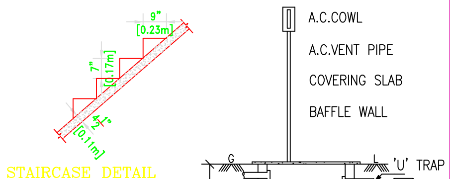
STAIRCASE DETAIL
