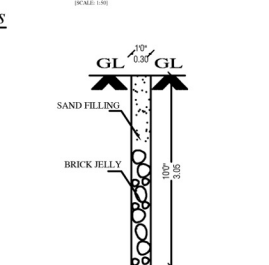
PERCOLATION PIT
