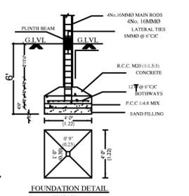
FOUNDATION DETAIL
