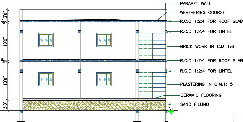
SECTION ON 'SC'
