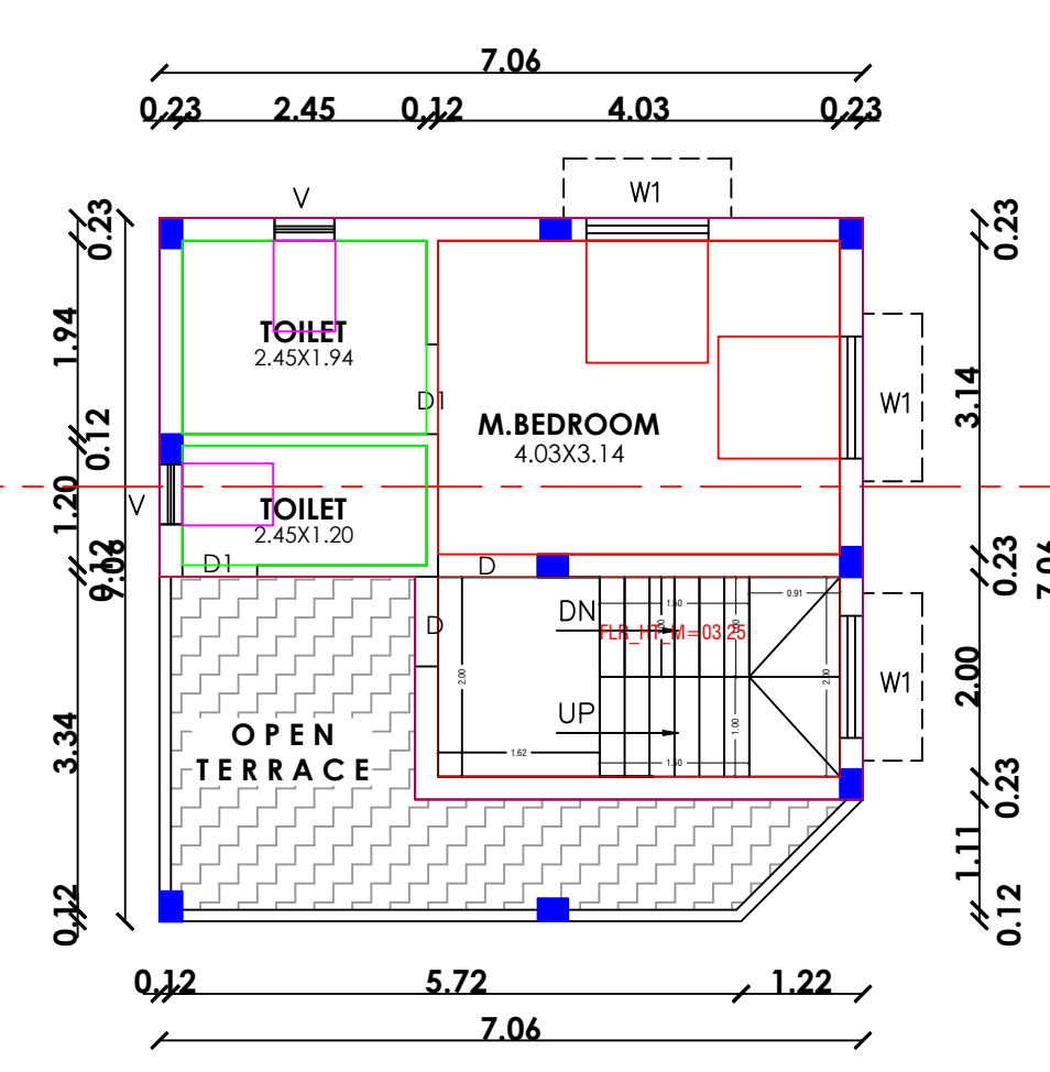
THIRD FLOOR PLAN (PROPOSED)
