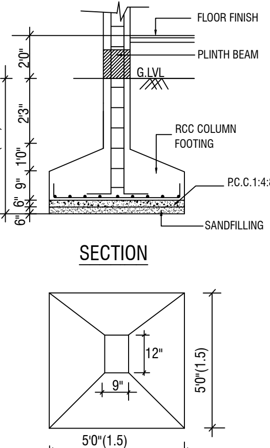
PLAN FOUNDATION DETAIL
