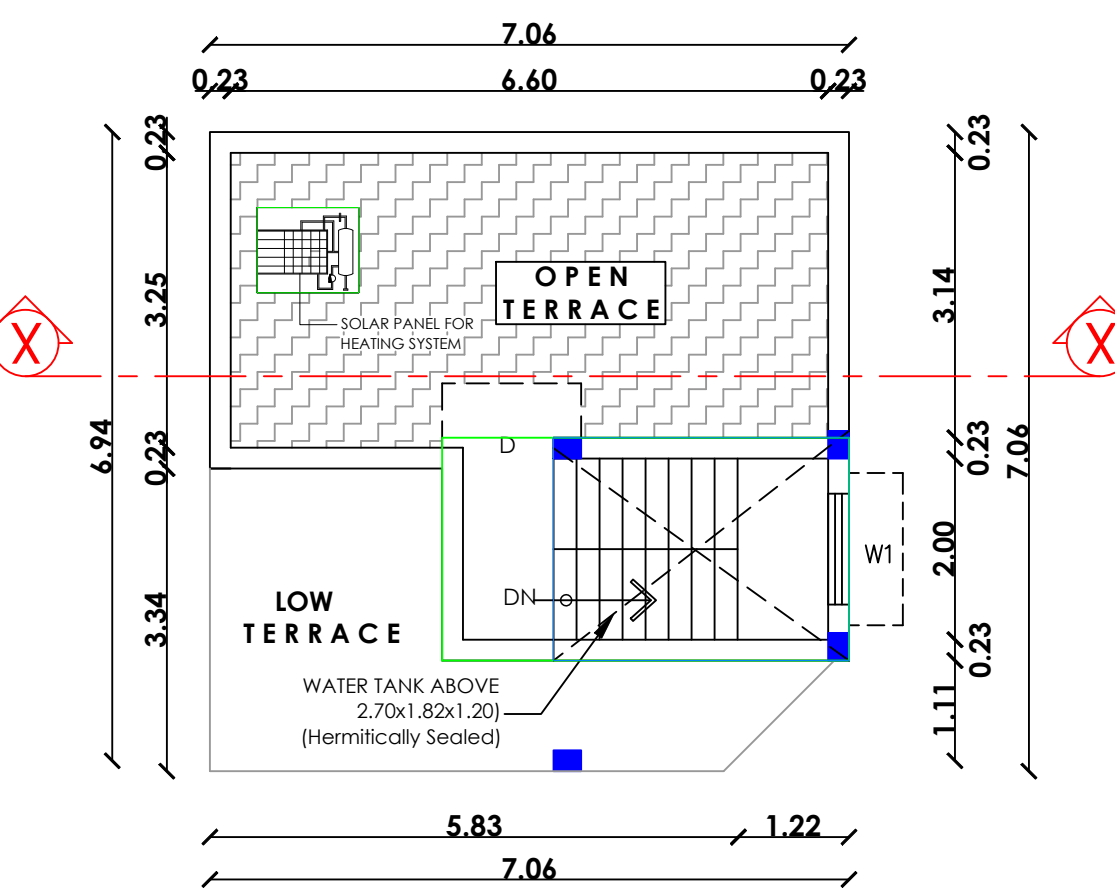
TERRACE FLOOR PLAN (PROPOSED)
