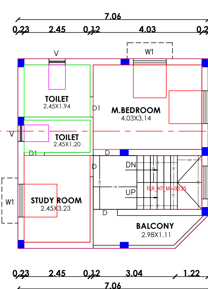
SECOND FLOOR PLAN (PROPOSED)
