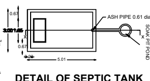
DETAIL OF SEPTIC TANK
