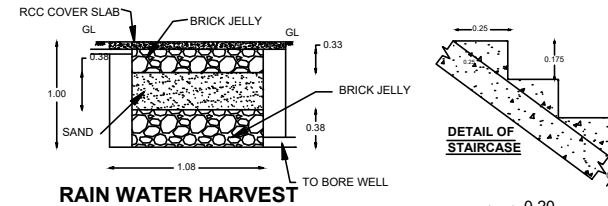
RAIN WATER HARVEST
