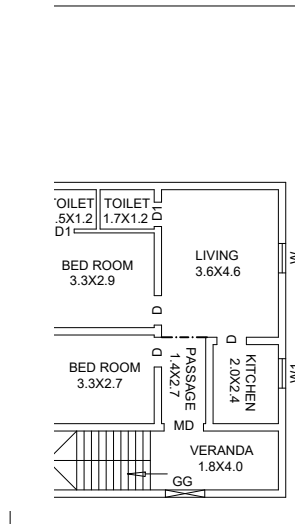
PROPOSED GROUND FLOOR
