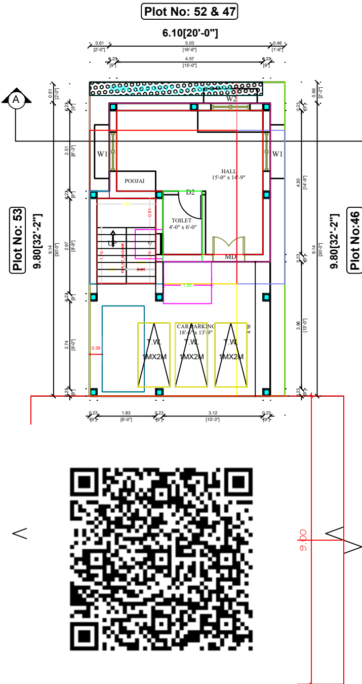
SITE CUM GROUND FLOOR PLAN
