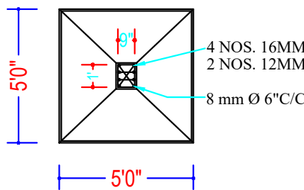
DETAIL OF COLUMN
