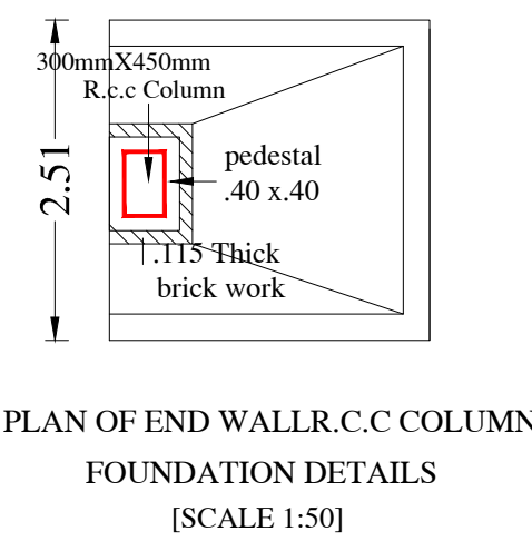
END WALL R.C.C COLUMN FOUNDATION DETAILS [SCALE 1:50]
