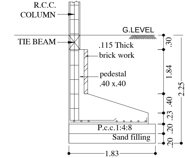
END WALL R.C.C COLUMN FOUNDATION DETAILS [SCALE 1:50]
