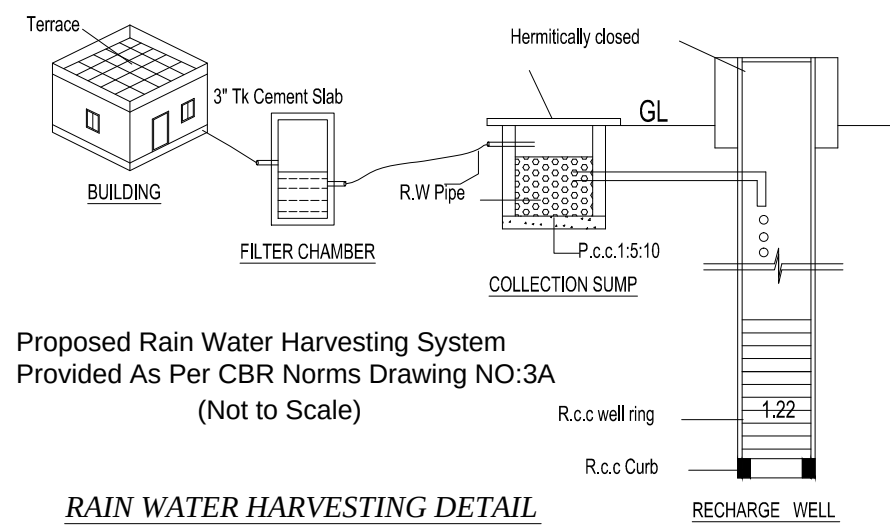
RAIN WATER HARVESTING DETAIL
