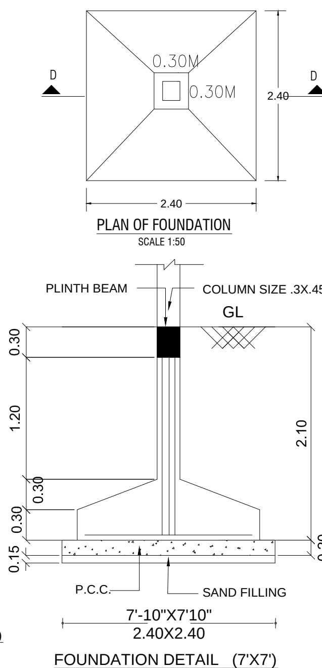
Footing Detail
