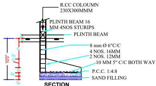
SECTION END WALL FOUNDATION
