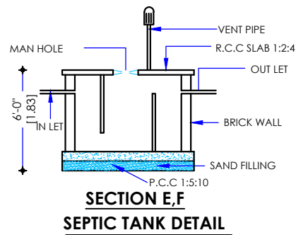
SECTION E.F SEPTIC TANK DETAIL
