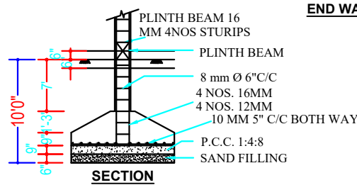
SECTION DETAIL OF COLUMN C1,C2
