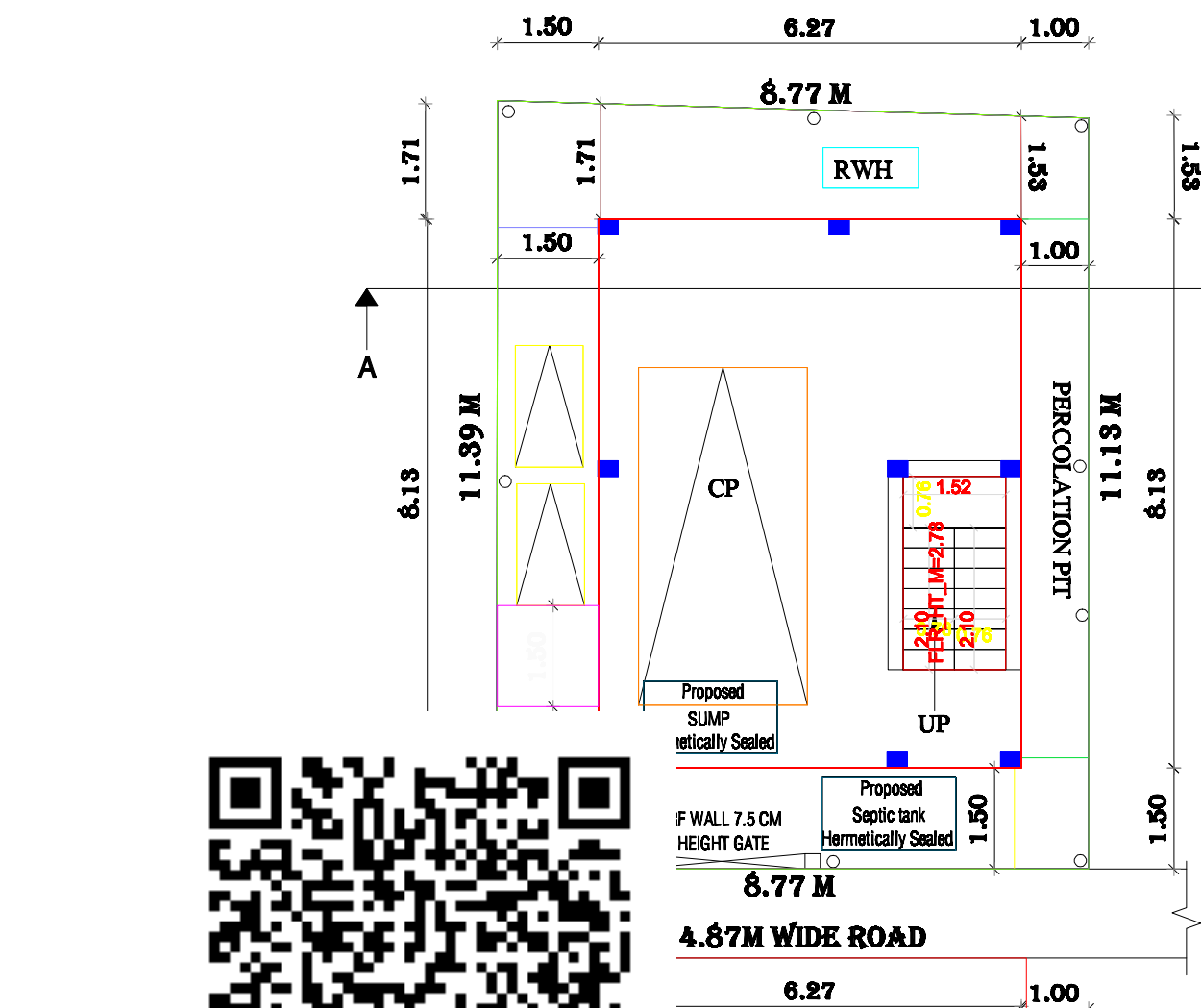
SITE CUM STILT FLOOR PLAN PROPOSED
