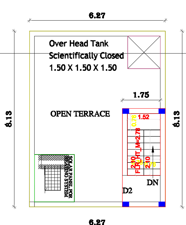
TERRACE FLOOR PLAN PROPOSED
