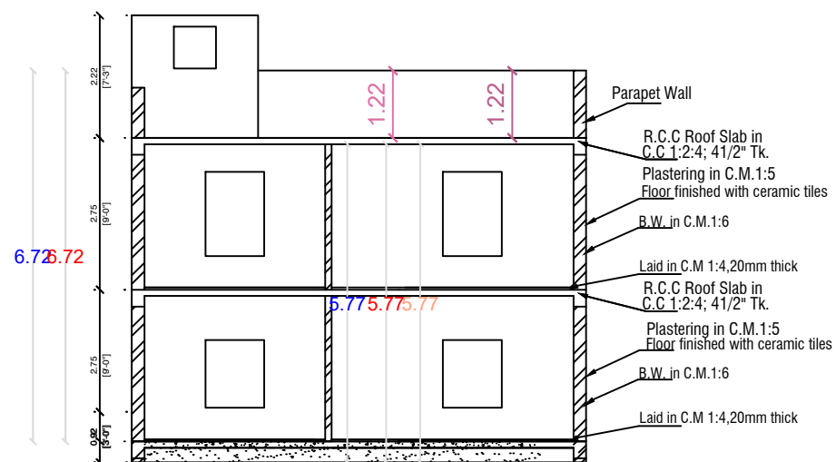
SECTION
