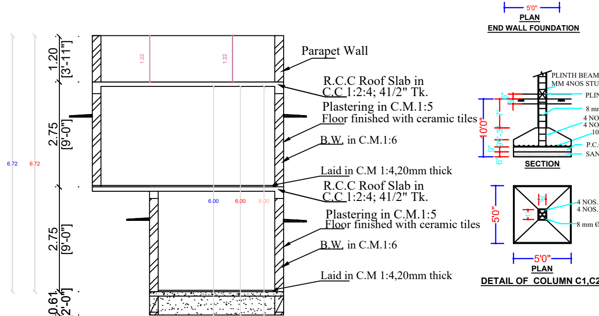
SECTION
