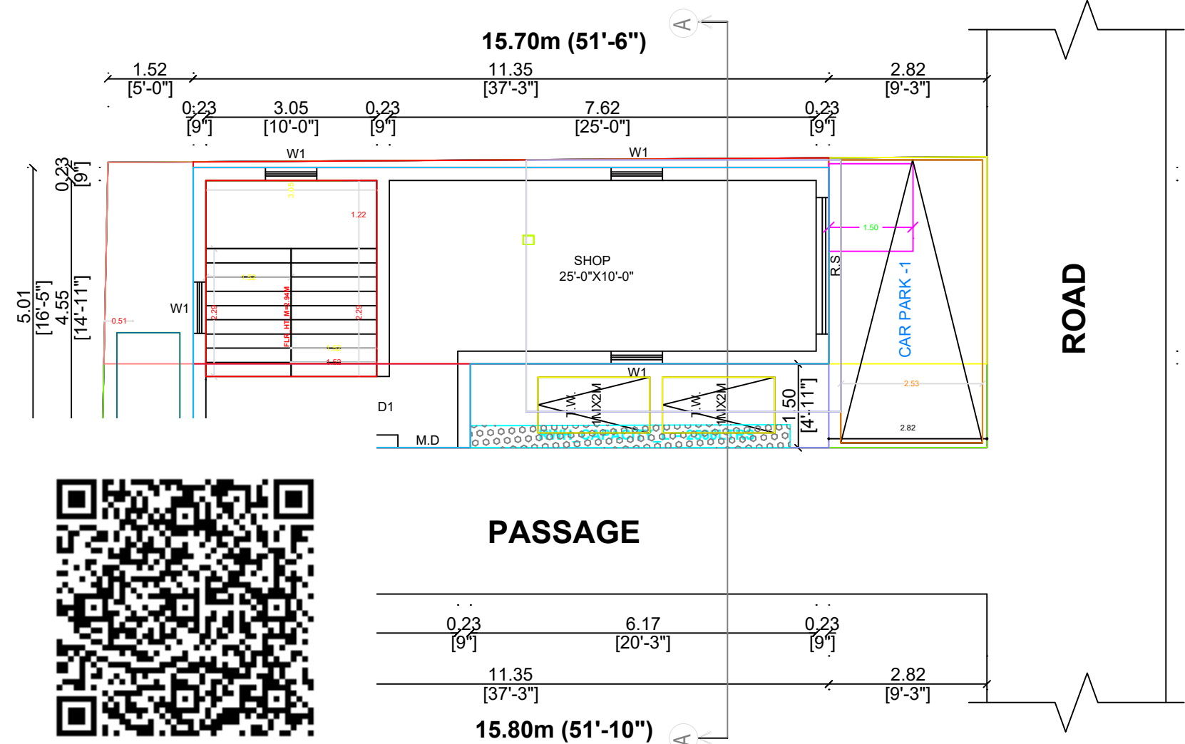
CUM GROUND FLOOR PLAN
