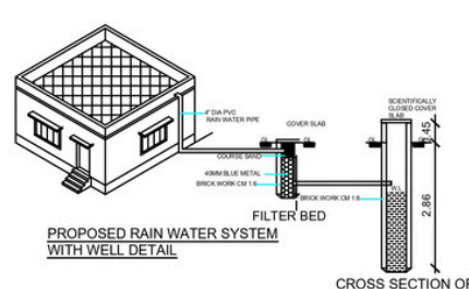
PROPOSED RAIN WATER SYSTEM WITH WELL DETAIL
