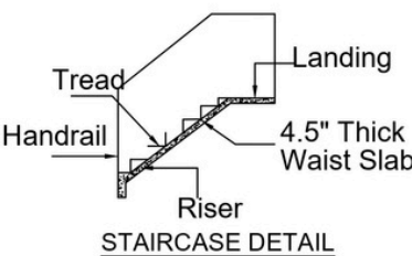
STAIRCASE DETAIL
