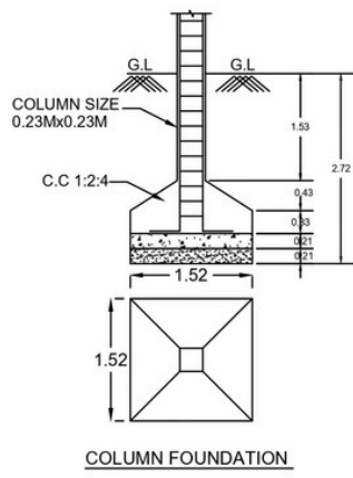
COLUMN FOUNDATION
