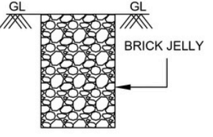
PERCOLATION PIT
