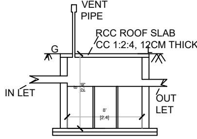
SECTION ON AA' AA'
