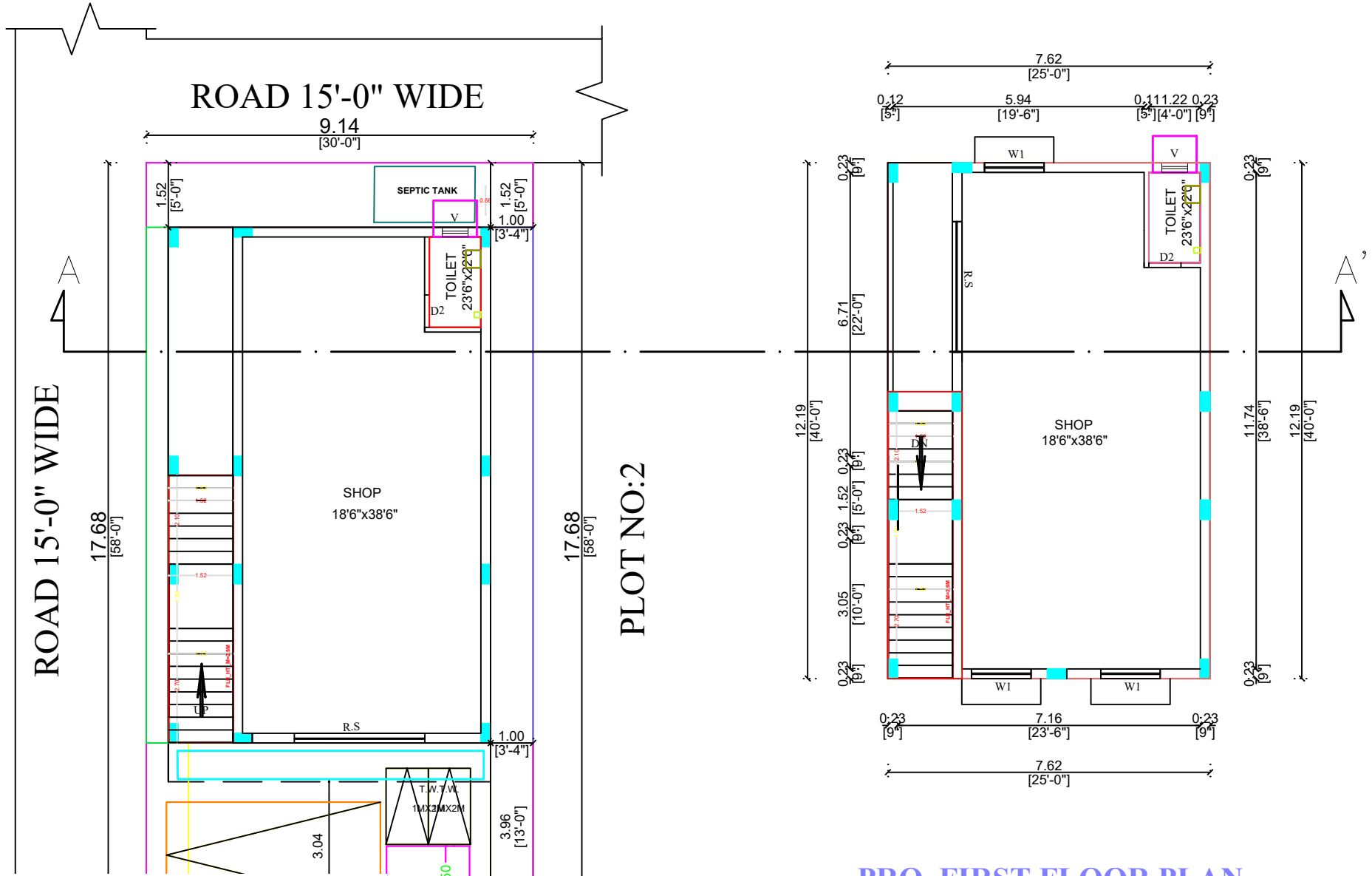
PRO. FIRST FLOOR PLAN
