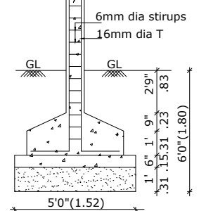
COLUMN FOUNDATION DETAIL
