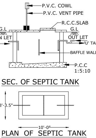
PLAN OF SEPTIC TANK
