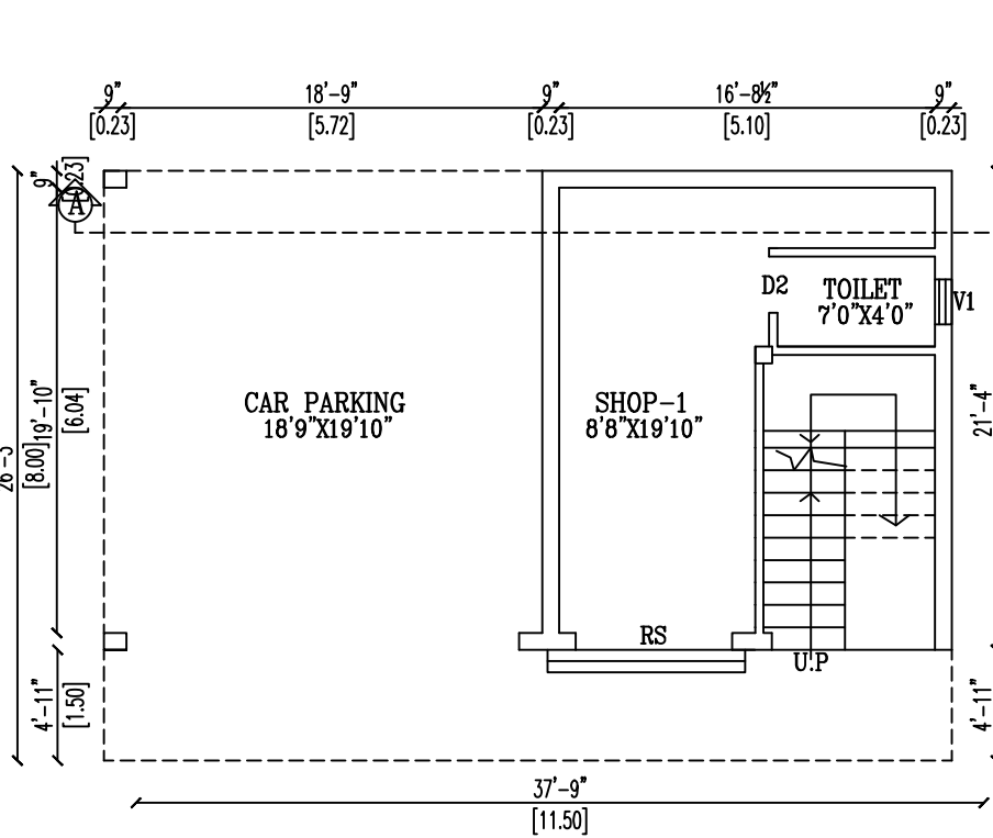
EXTG. GROUND FLOOR PLAN
