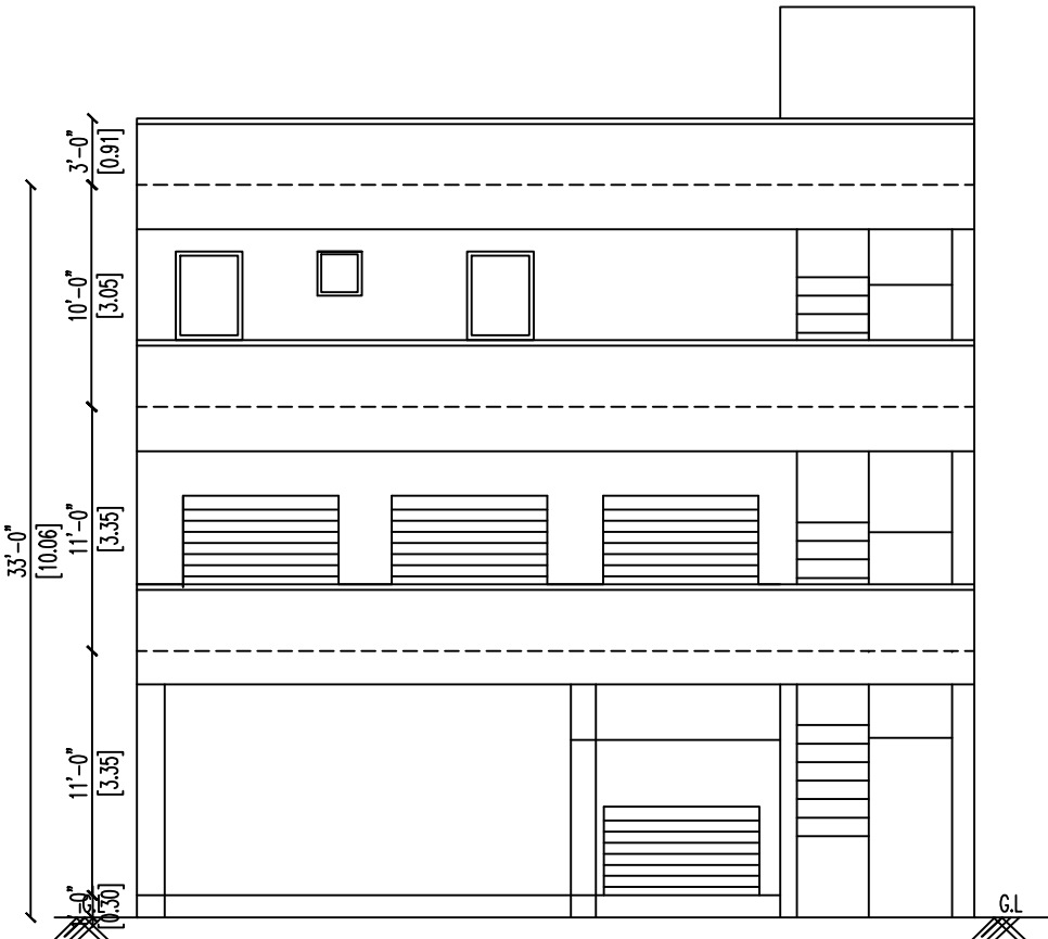
FRONT ELEVATION
