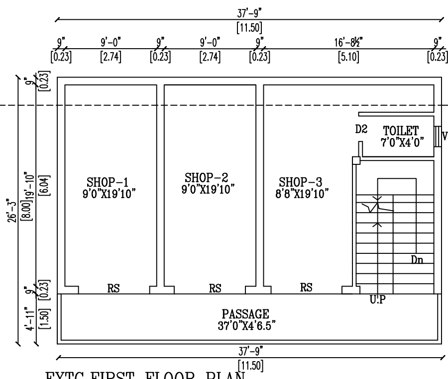
EXTG.FIRST FLOOR PLAN
