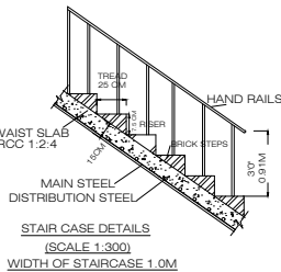
STAIR CASE DETAILS (SCALE 1:300) WIDTH OF STAIRCASE 1.0M
