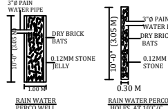
DETAILS OF RAIN WATER HARVESTING SYSTEM
