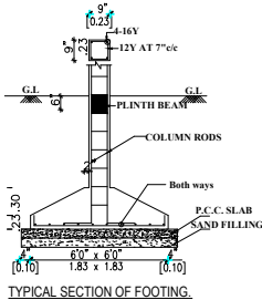
TYPICAL SECTION OF FOOTING.
