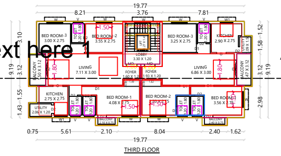
THIRD FLOOR
