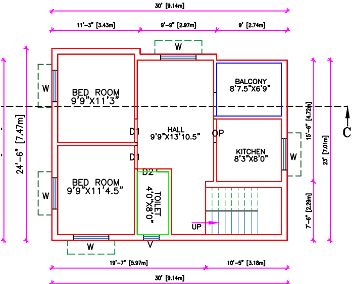
TYPICAL FIRST & SECOND FLOOR
