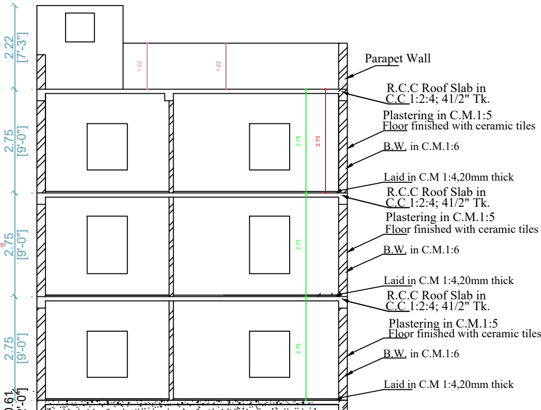
SECTION
