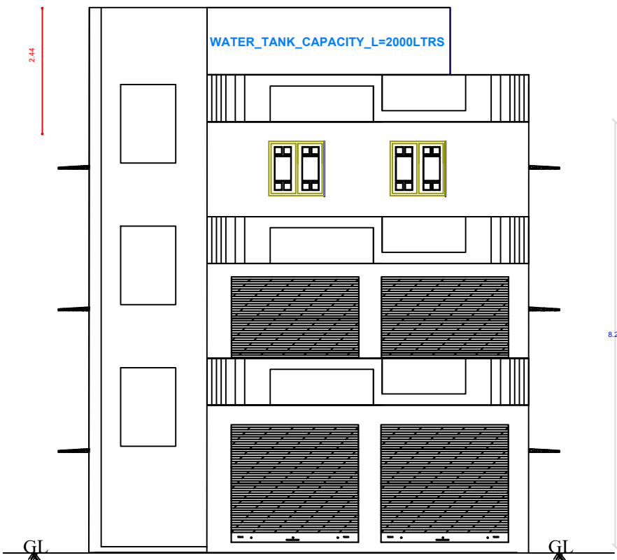
FRONT ELEVATION
