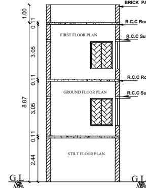
SECTION-YY
