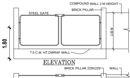
PLAN COMPOUND WALL DETAILS (NOT TO SCALE)
