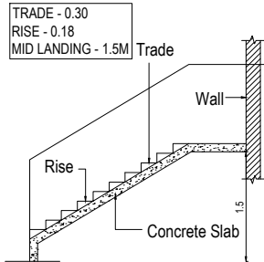
STAIR DETAILS
