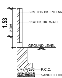
SECTION OF GATE (NOT TO SCALE)
