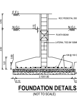
FOUNDATION DETAILS (NOT TO SCALE)
