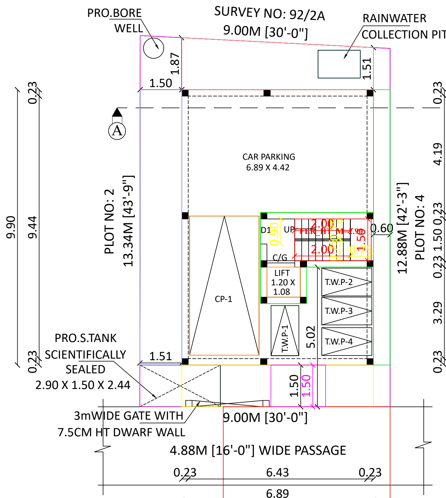
PRO.STILT FLOOR PLAN
