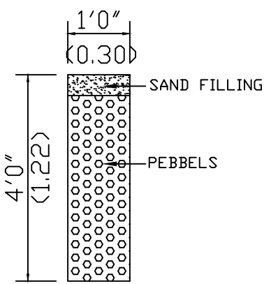
PERCOLATION PIT (Not To Scale)
