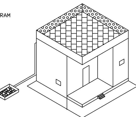
RAIN WATER HARVESTING CHAMBER (Not To Scale)
