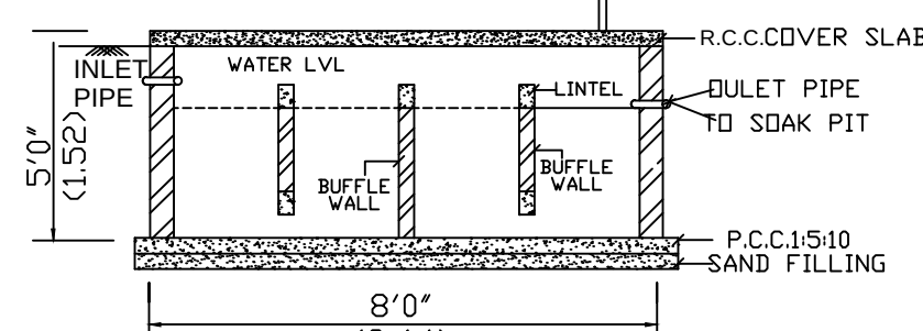
SEPTIC TANK SECTION (Not To Scale)
