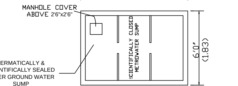
PLAN OF SUMP (Not To Scale)
