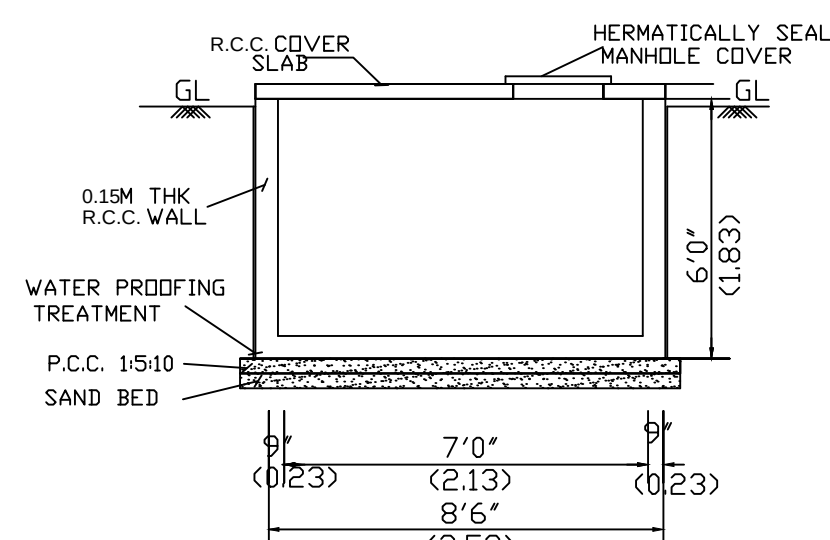
SECTION OF SUMP (Not To Scale)
