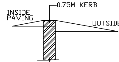
DWARF WALL SECTION (Not To Scale)
