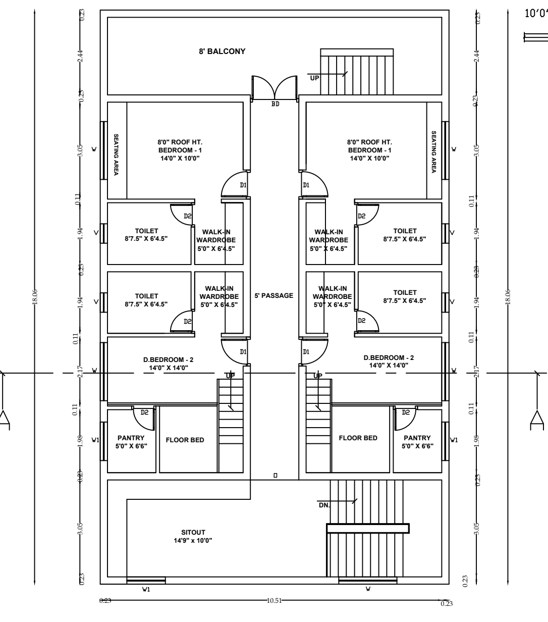
FIRST MEZZANINE FLOOR PLAN
