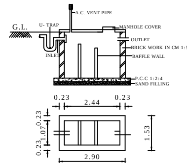
SEPTIC TANK DETAIL
