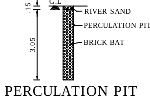
PERCOLATION PIT
