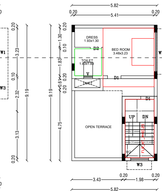
SECOND FLOOR PLAN (PROPOSED)
