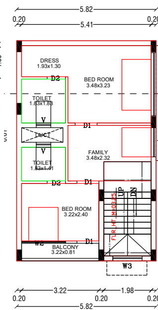
FIRST FLOOR PLAN (PROPOSED)
