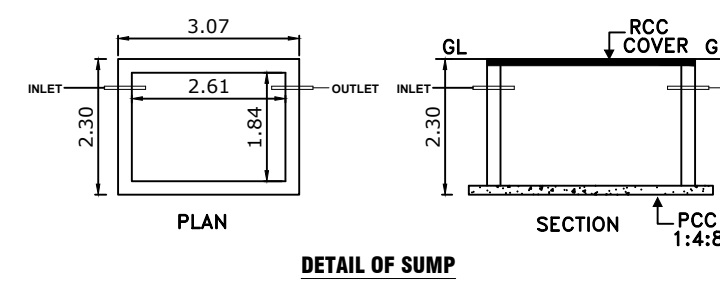
DETAIL OF SUMP
