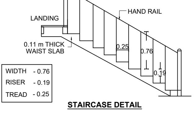
STAIRCASE DETAIL
