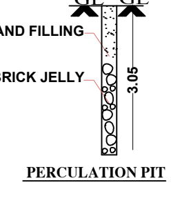
PERCOLATION PIT
