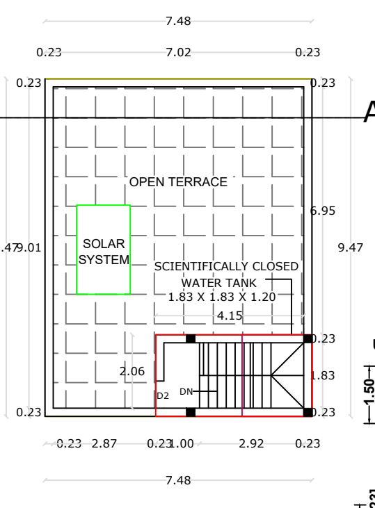
TERRACE FLOOR
