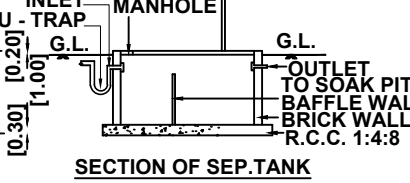
SECTION OF SEP. TANK
