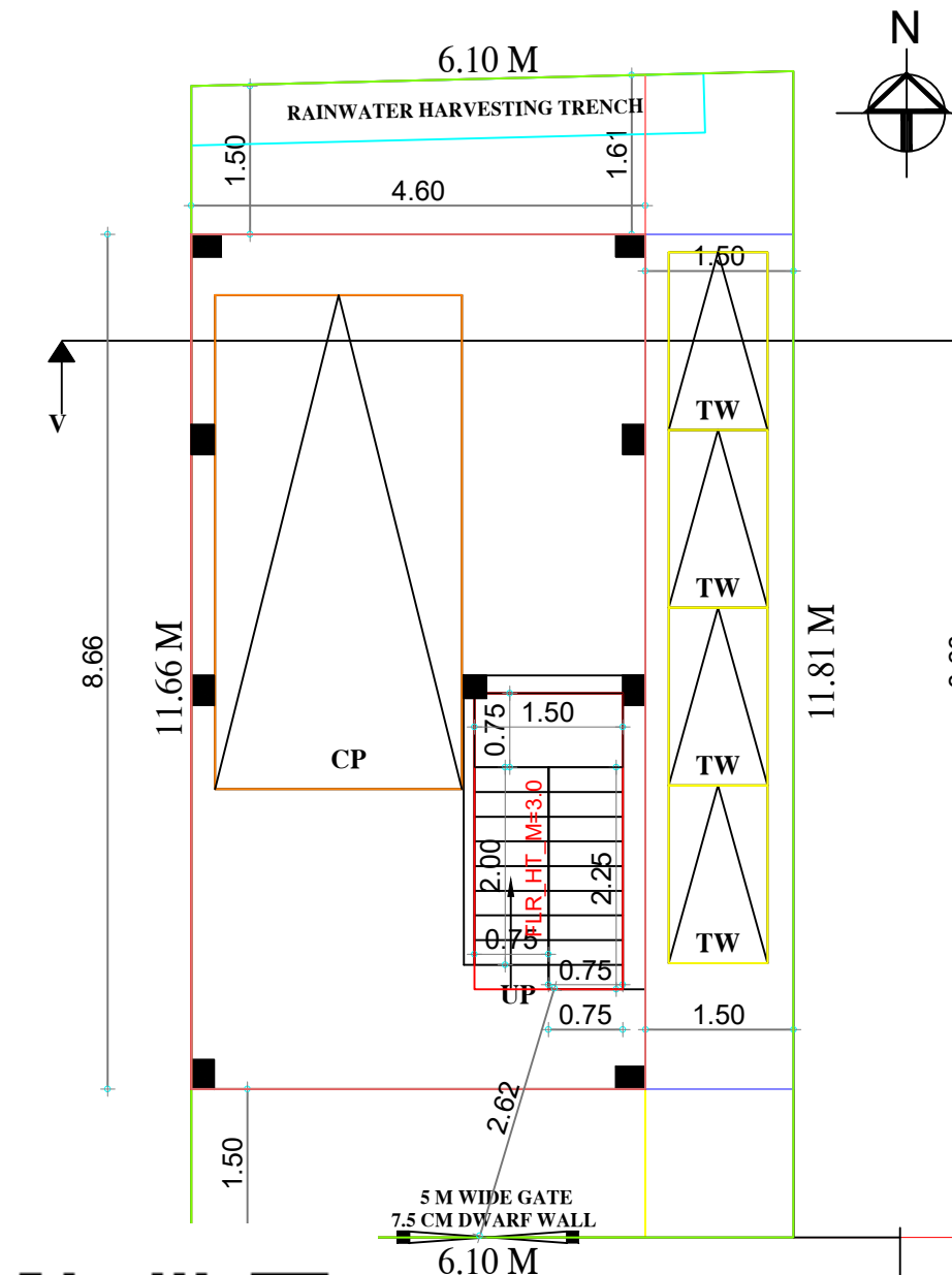
UM STILT FLOOR PLAN (PROPOSED)
