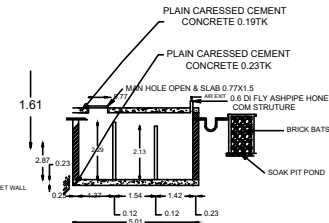
SECTION XX
