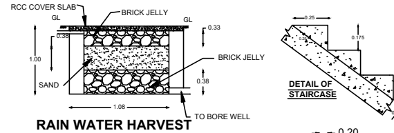
RAIN WATER HARVEST
