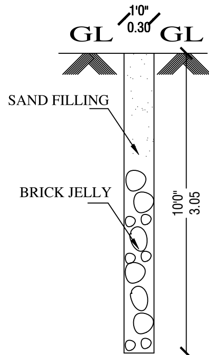
PERCULATION PIT
