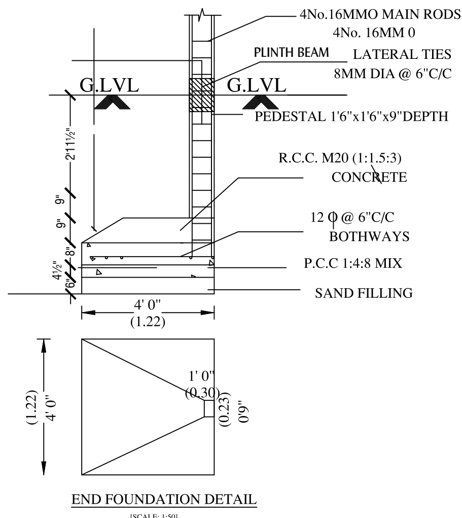
END FOUNDATION DETAIL
