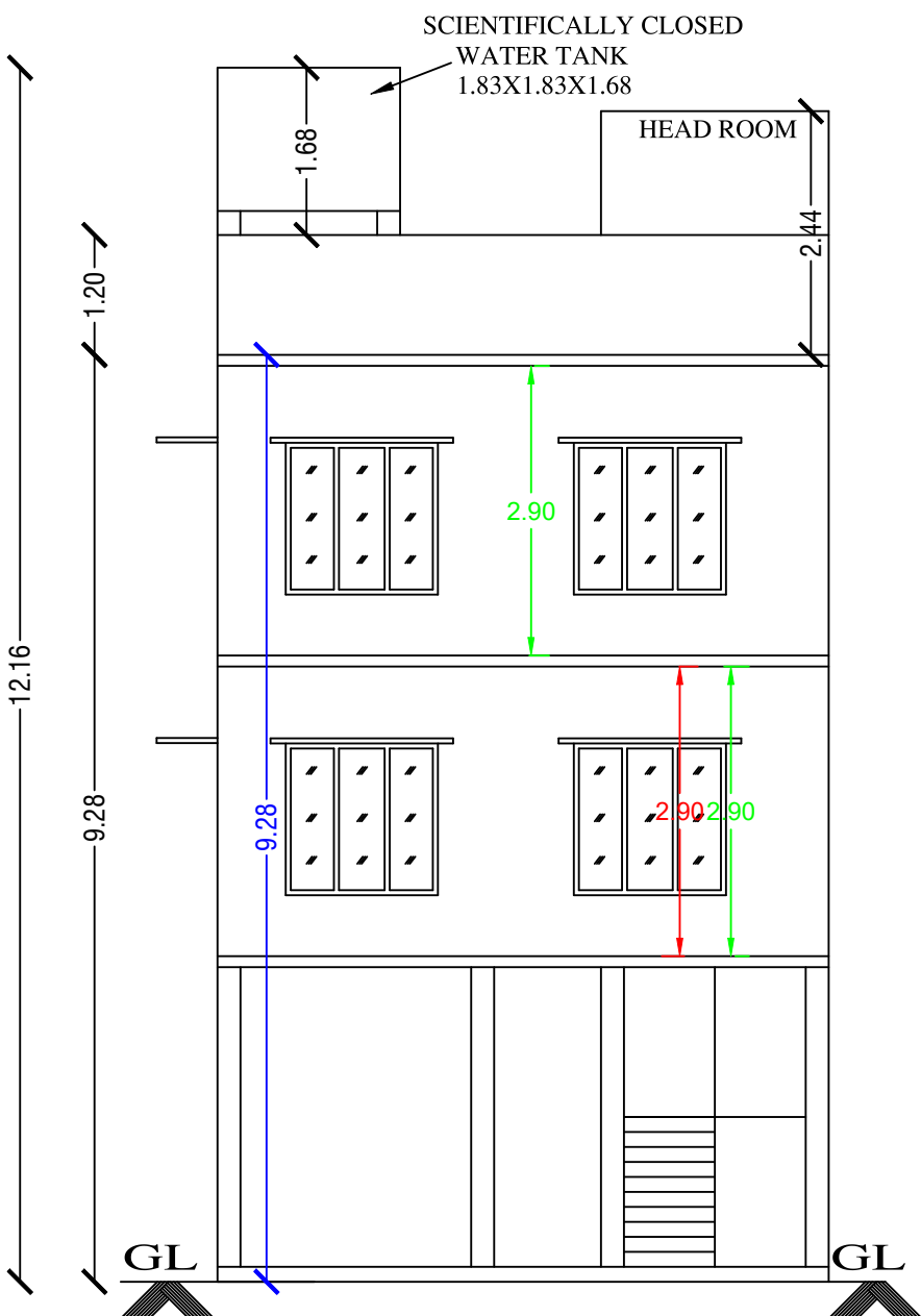
FRONT ELEVATION
