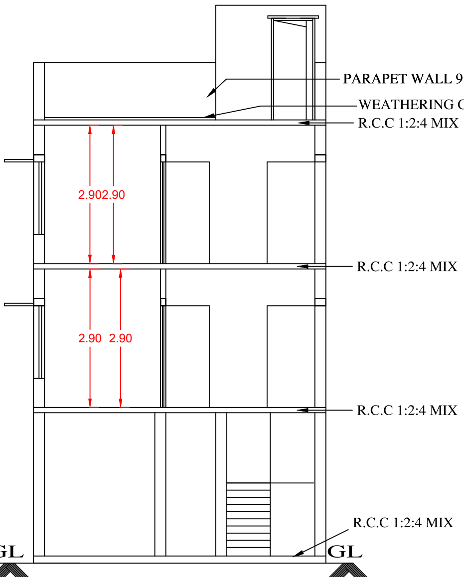
SECTION : "A-A"
