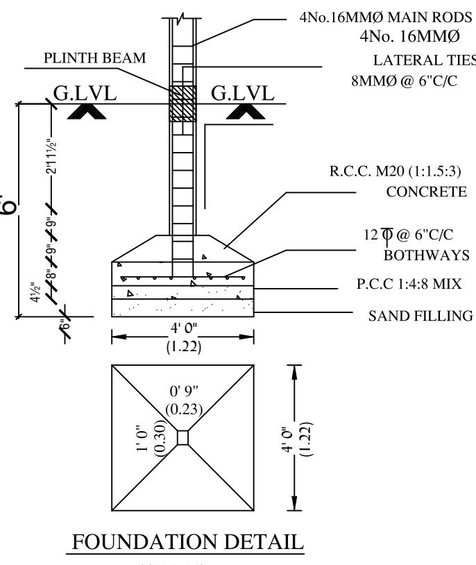
FOUNDATION DETAIL
